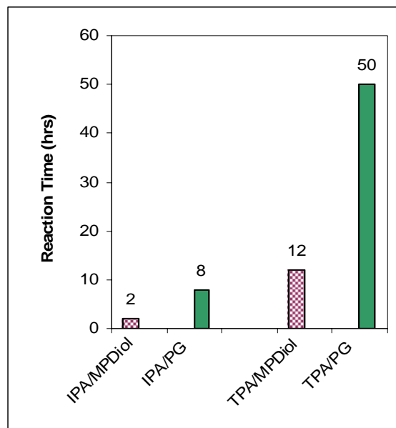
Figure 2. Comparative reaction rates of PG and MPDiol glycol with isophthalic and terephthalic acid
