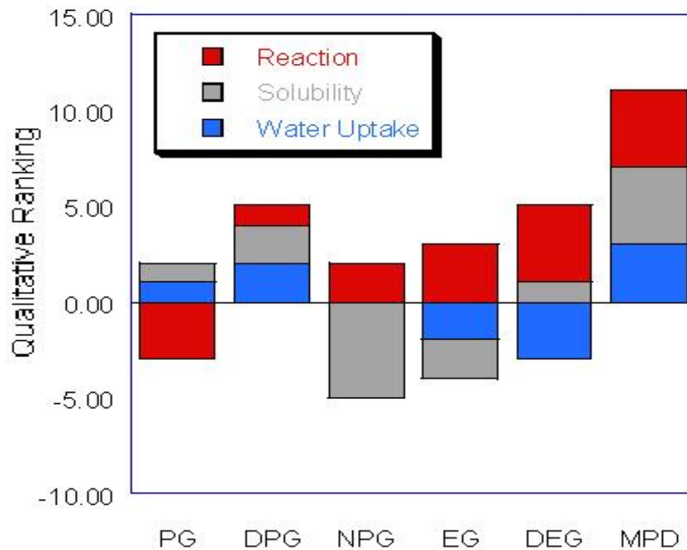
Figure 3. Comparison of TPA-glycol reactions incorporating factors for reaction rates, polymer solubility in styrene and water absorption of UPR.
