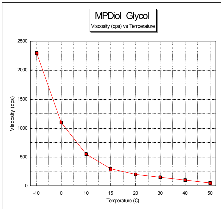
Viscosity Vs. Temperature Chart
