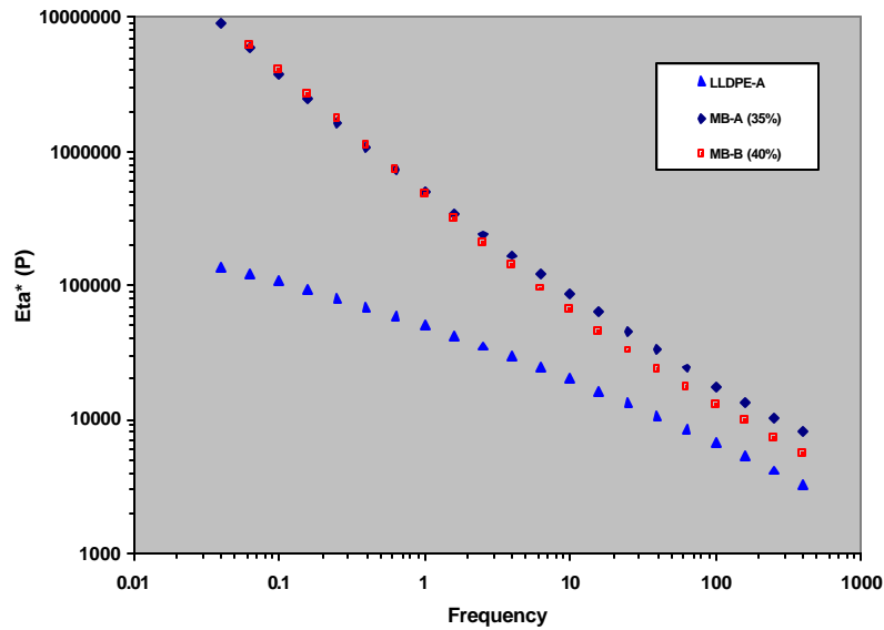
Figure 1. Complex viscosity vs. frequency for LLDPE-A, MB-A, and MB-B at 230°C
