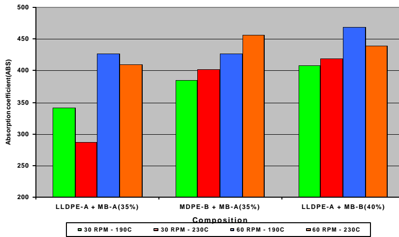
Figure 3. ABS vs. screw speed for the jacket blends extruded at 190 °C and 230 °C
