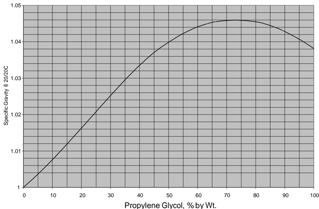
Specific Gravity of Aqueous Propylene Glycol Solutions
