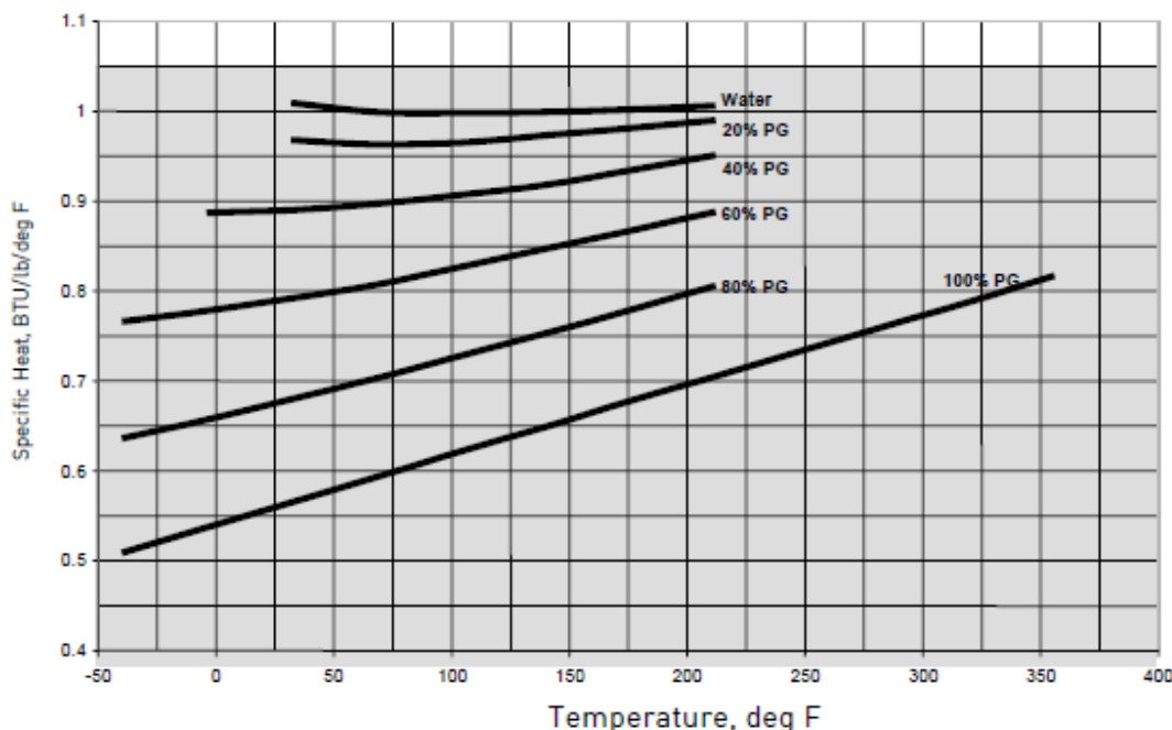
Specific Heat of Aqueous Propylene Glycol Solutions
