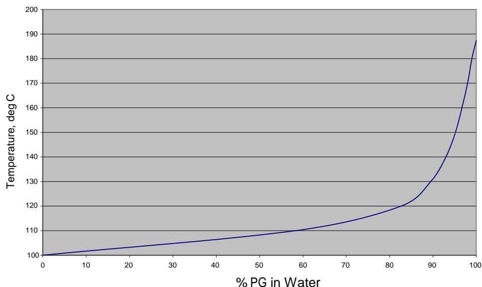
Boiling Point of Propylene Glycol/Water Mixtures
