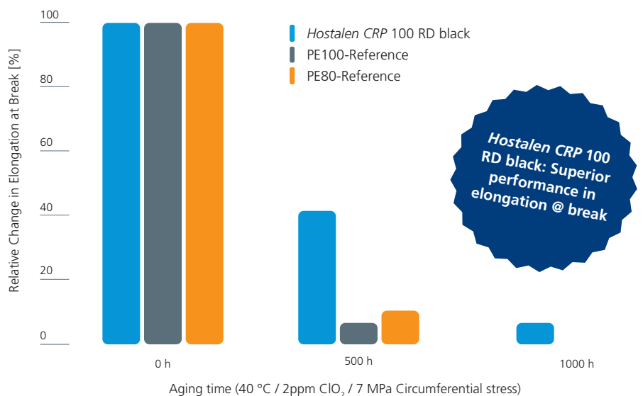
NOL ring test after "stressed" aging in ClO 2
